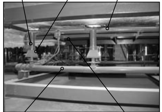
Burner Manifold Figure 34 Ignition Bar Pilot & Thermocouple
